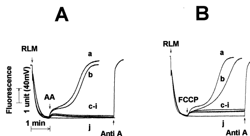
Fig. 1. Mitochondrial membrane potential collapse induced by AA and FCCP: the effects of ADP, catalase, carboxyatractylolide, DTT, EGTA, CsA and rotenone. RLM (0.5 mg ml -1 ) were incubated in medium containing 125 mM sucrose, 65 mM KCl, 10 mM HEPES, pH 7.2, 2 mM \text{KH}_2\text{PO}_4 , 1 mM \text{MgCl}_2 , 5 mM sodium succinate, 30 \mu\text{M} \text{CaCl}_2 and 5 \mu\text{M} safranin, at 30°C. As indicated, 10 \mu\text{M} AA (panel A, line a) or 50 nM FCCP (panel B, line a) was added in the presence of 1 \mu\text{M} carboxyatractylolide (lines b), 200 nmol ADP and 2 \mu\text{g} oligomycin ml -1 (lines c), 2.0 \mu\text{M} catalase (lines d), 2 mM DTT (lines e), 1 mM EGTA (lines f), 1.0 \mu\text{M} CsA (lines g), 4 \mu\text{M} rotenone (lines h) or 5 mM \beta -hydroxybutyrate plus 0.1 mM isocitrate (lines i). Lines j represent control experiments without additions. Antimycin A (1 \mu\text{g} ml -1 ) was added at the end of the experiments.
